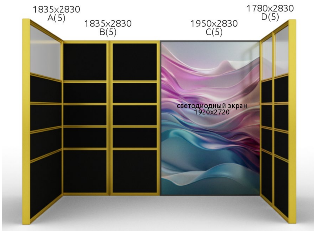
LED-panel 960x1360px / 1920x2720mm
